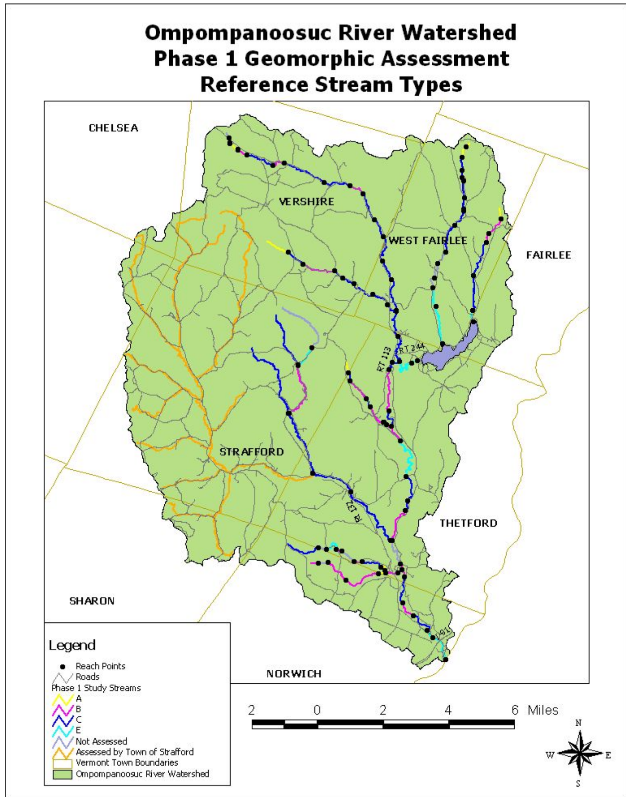
Figure 5. Reference Stream Types within the Ompompanoosuc River Watershed
